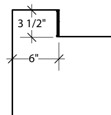
3" FLATLITE® DFL-0300X in ADT-0300C Track
